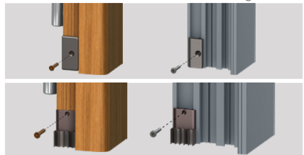
Smooth frame
